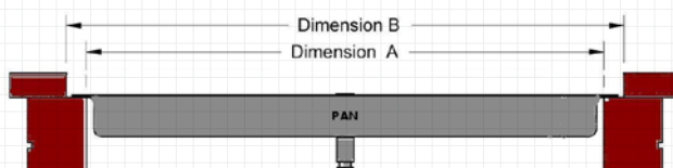
Recessed Mount
